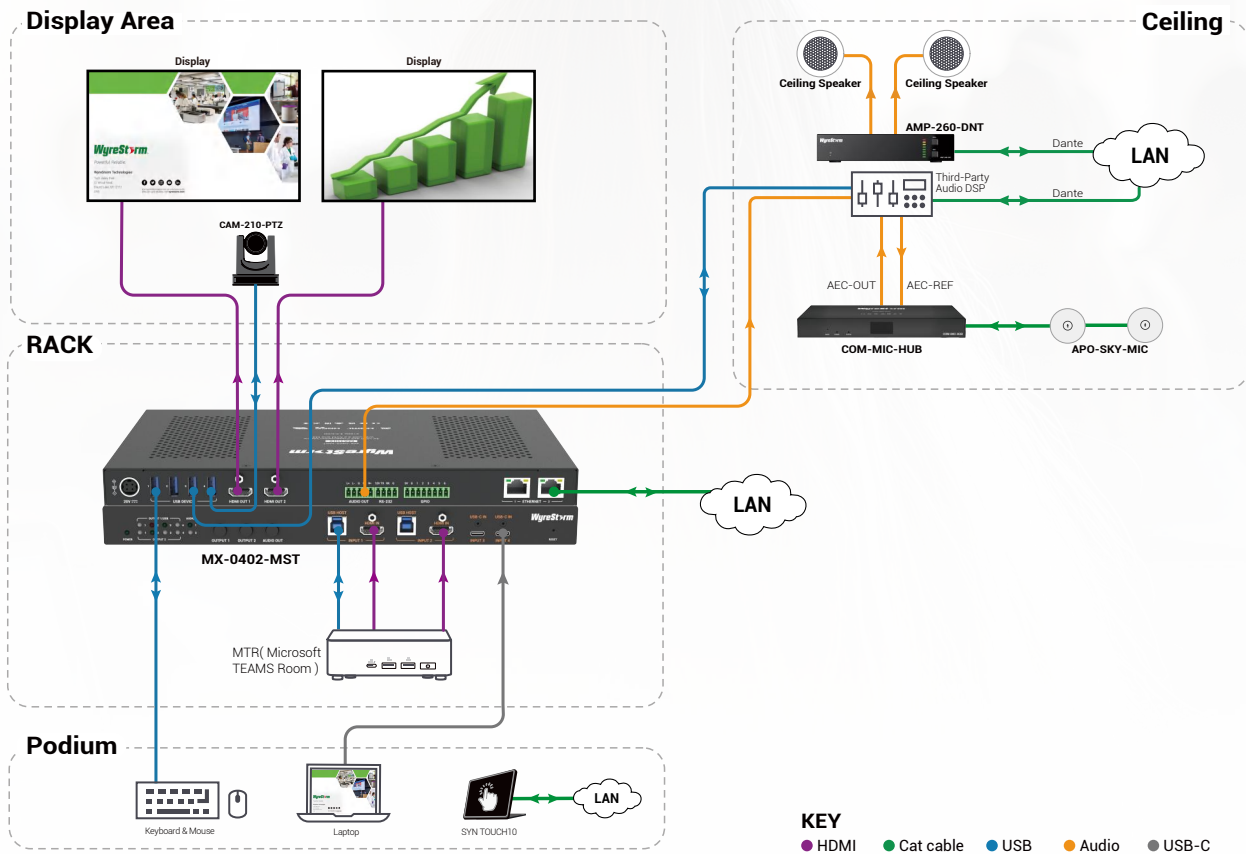
Medium & Multi-Functional Classroom Solution MX-0402-MST (With MTR)
