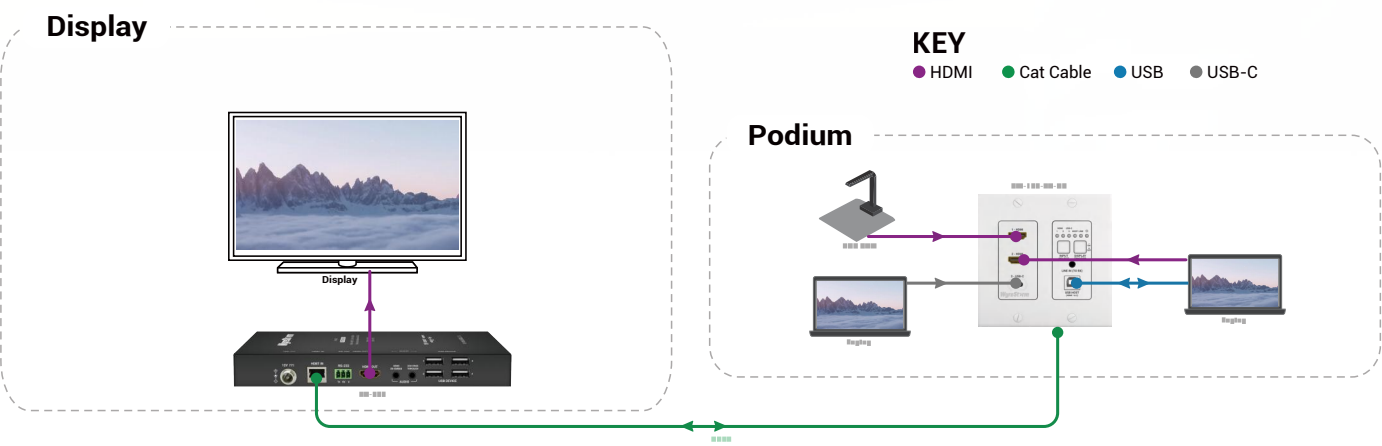
Plug-and-play, Small & Medium Classroom SW-130-TX & RX-500 (Budget:Standard)
