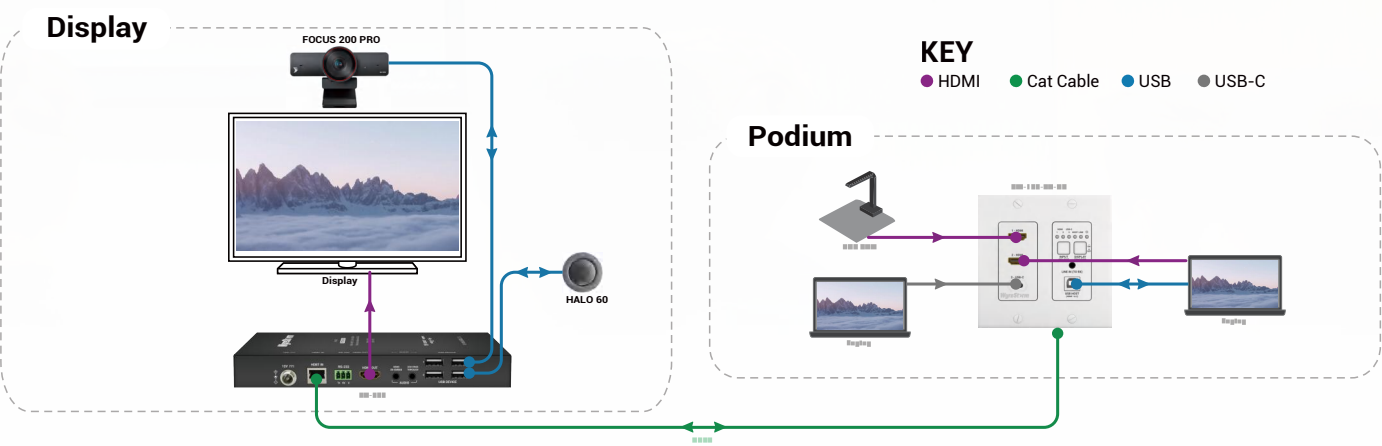
Plug-and-play, Small & Medium Classroom SW-130-TX & RX-500 (Budget:Hybrid)
