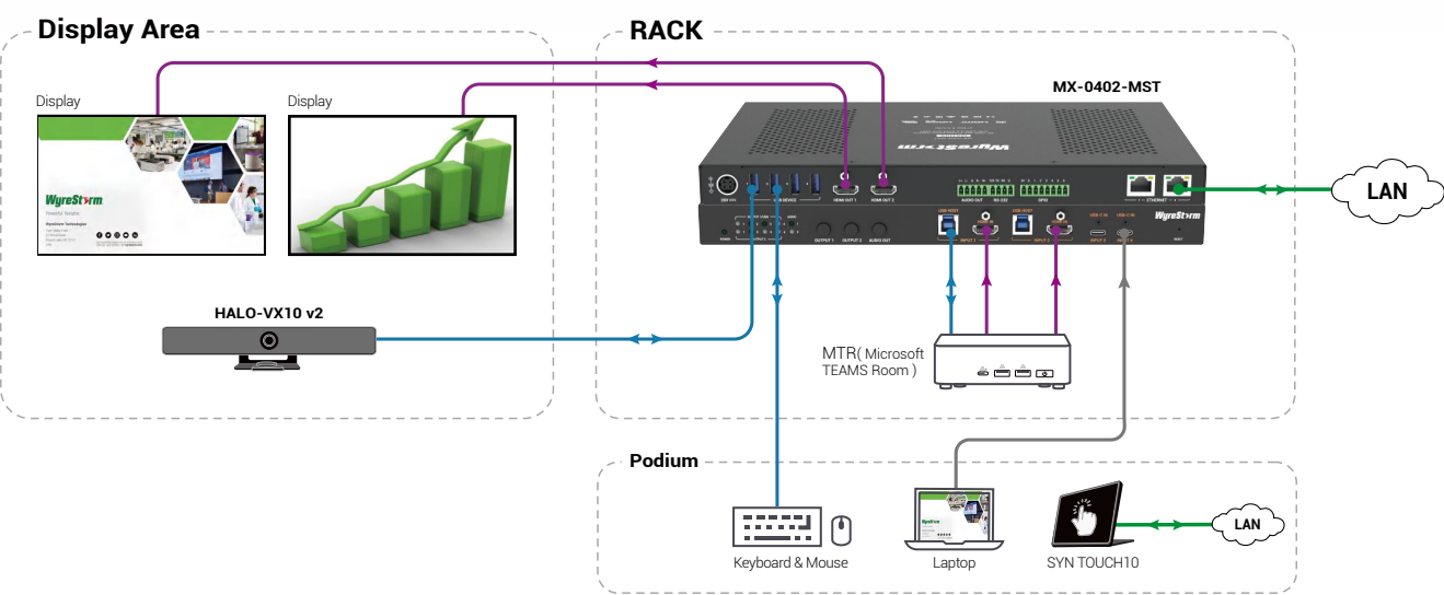
Small Multi-Functional Classroom Solution MX-0402-MST (With MTR)
